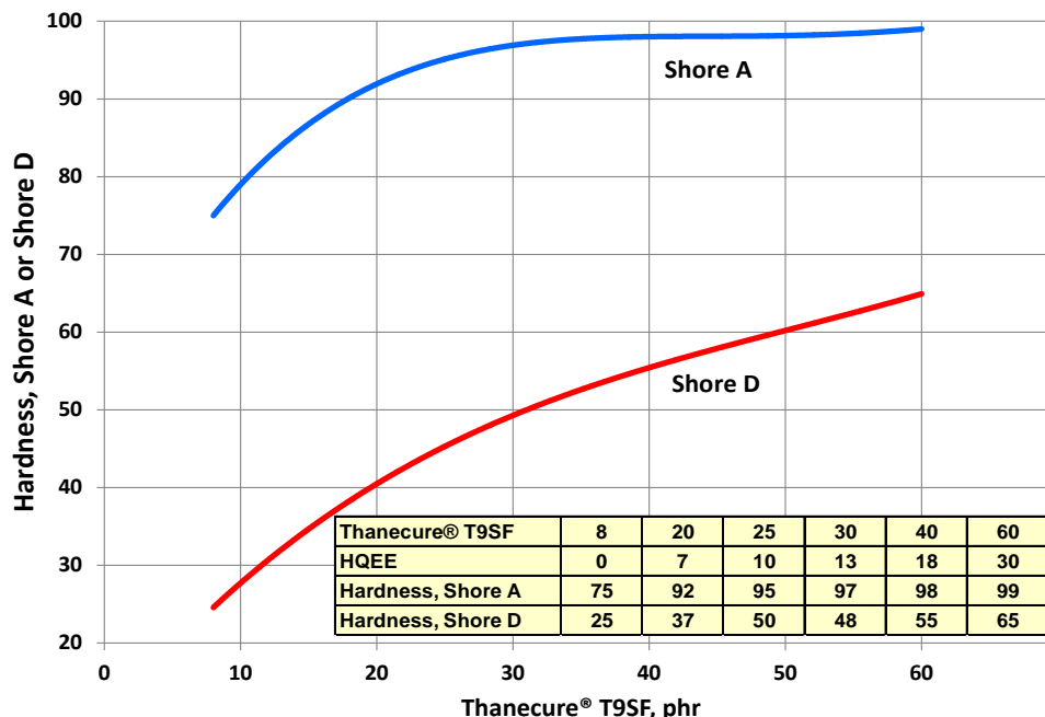
Millathane® 26 - Isocyanate Cures Hardness vs. Thanecure® T9SF/HQEE Levels
